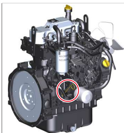
Fig. 240: 3TNV88-BKWN (DW30)
